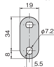
板厚 t=2.3 Plate thickness
