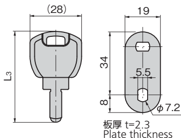
止め金(兼用型) Stopper plate (combined-use type)
