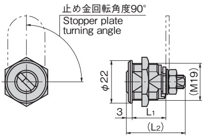
止め金(兼用型) Stopper plate (combined-use type)
